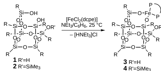
Scheme 1. Synthesis of the mono iron compounds, R = c -C 5 H 9 .
